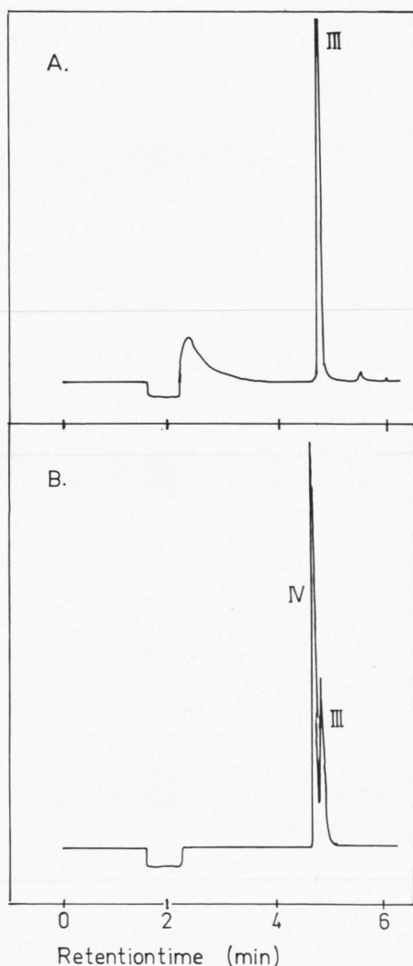
Fig. 1. Separation of 7 S -heliotrine and its metabolites by capillary GLC. A. 7 S -heliotrine; B. alkaloid extract from C. transiens , after application of 7 S -heliotrine.
