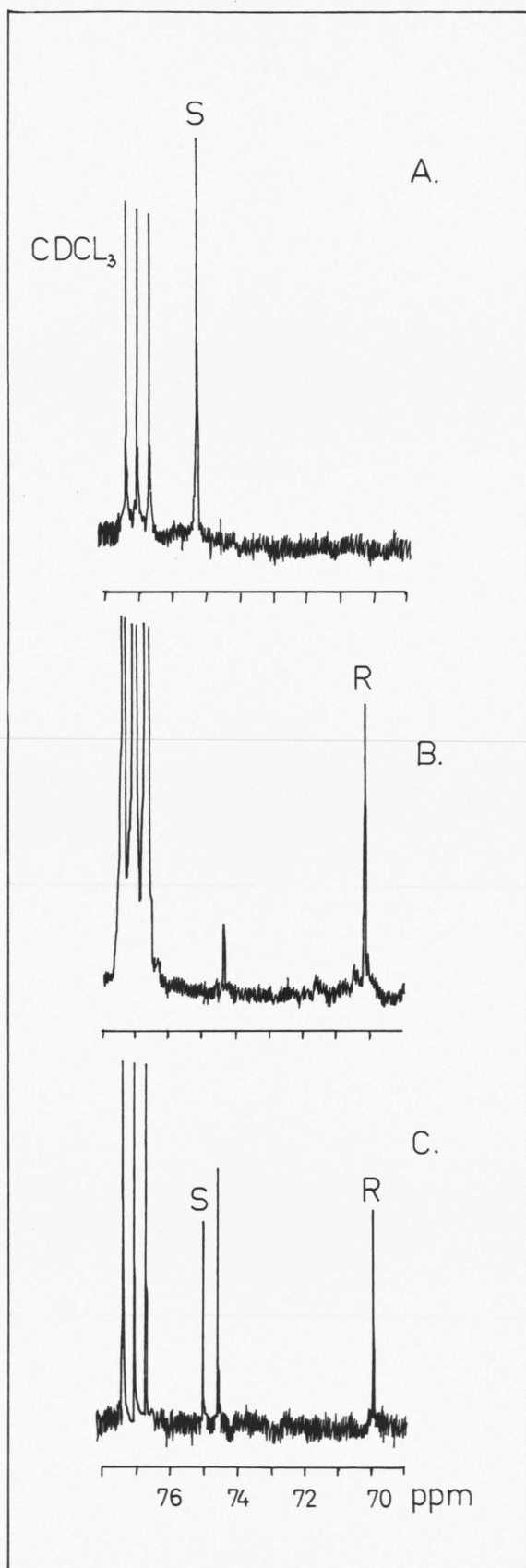
Fig. 2. ^{13}\text{C} NMR analysis of 7 S -heliotrine and its metabolites. A. 7 S -heliotrine; B. 7 R -heliotrine*, the metabolite from S. transiens ; C. racemization product of 7 S -heliotrine in \text{CDCl}_3 .
